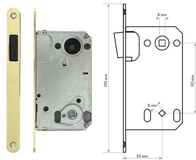
Privacy set lock
