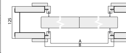
DOUBLE POCKET DOOR for dry walls
