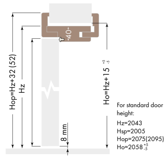
Rebated doorframe
