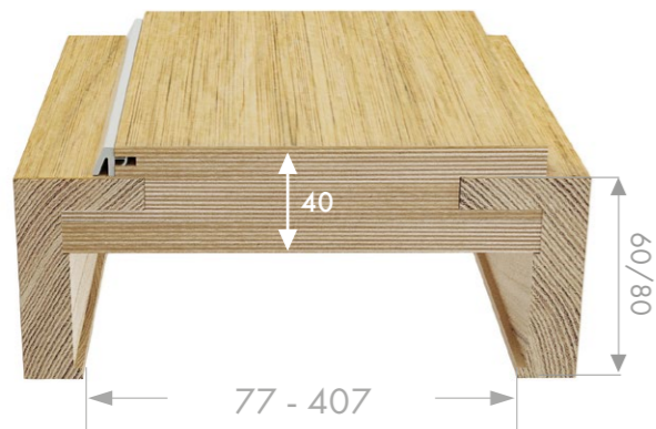
Adjustable doorframe BASIC
