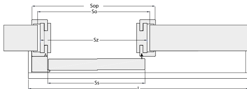
Single Wall-Mounted Sliding System
