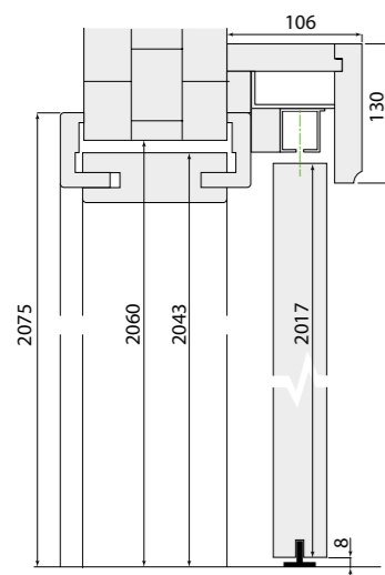
Wall-Mounted Sliding System
