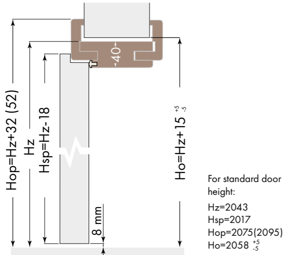
Doorframe with a panel
