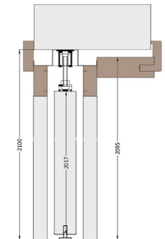
SINGLE POCKET DOOR wall mounted with a top mounting track
