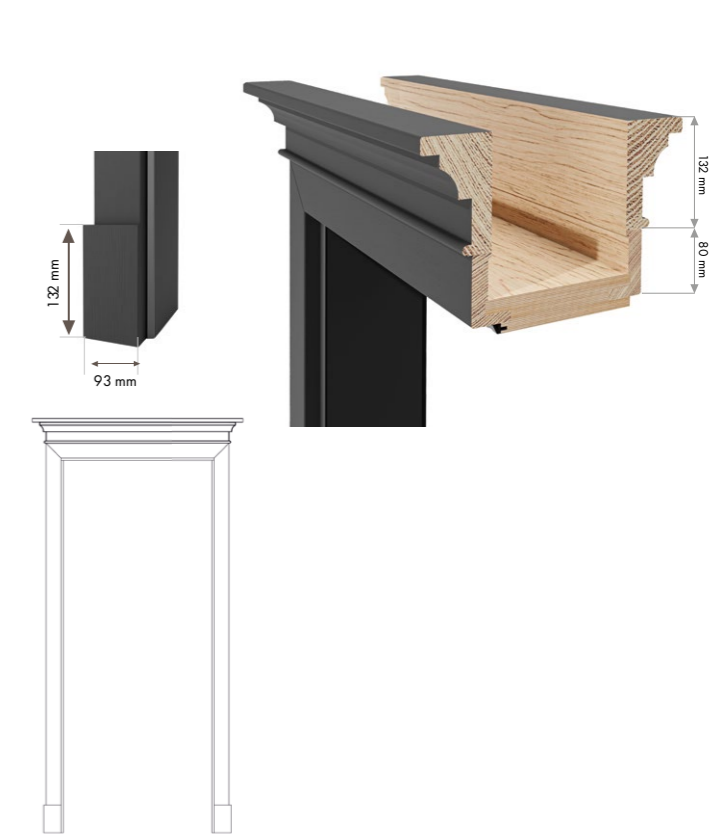
8. Adjustable doorframe with a washboard and a crown moulding
