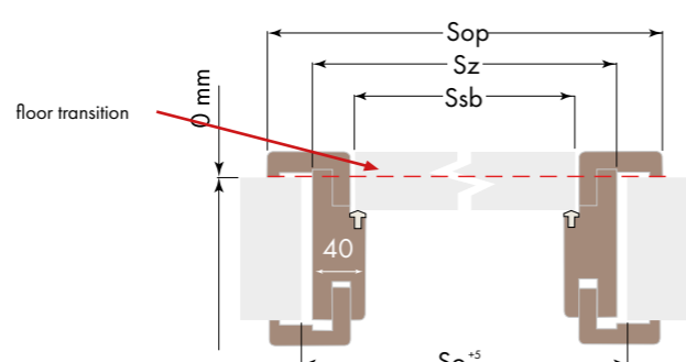
Adjustable doorframe (non-rebated door)
