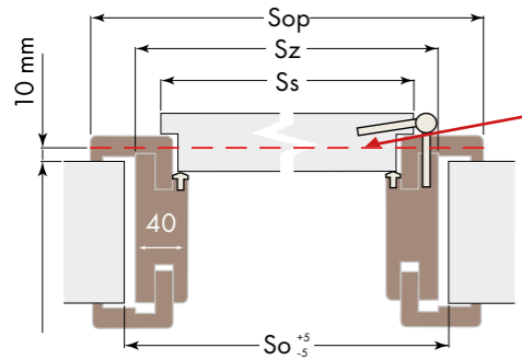
Adjustable doorframe (rebated door)
