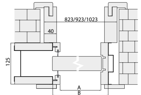
SINGLE POCKET DOOR wall mounted with a top mounting track
