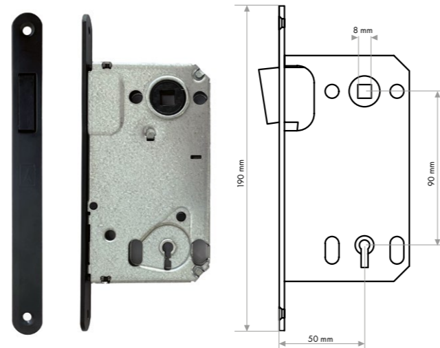
Key-operated lock
