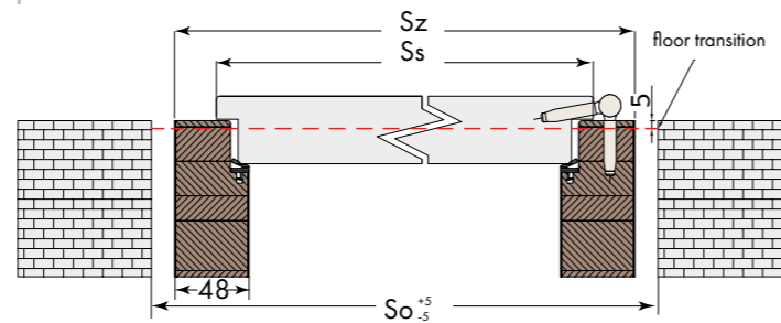
Rebated doorframe
