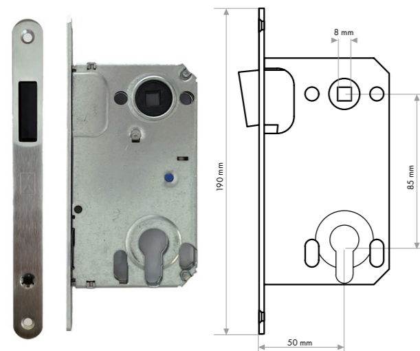
Cylinder-operated lock
