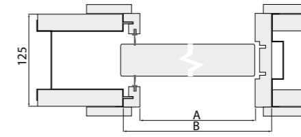
SINGLE POCKET DOOR for dry walls
