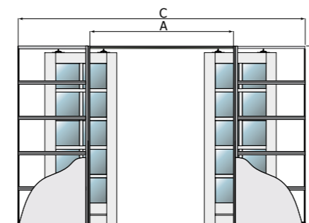
DOUBLE POCKET DOOR for dry walls
