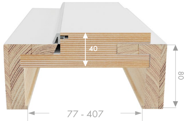
Adjustable doorframe SOFT
