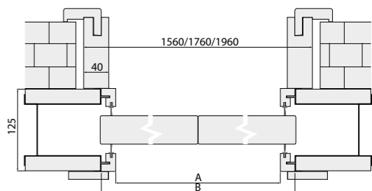
DOUBLE POCKET DOOR wall mounted with a top mounting track
