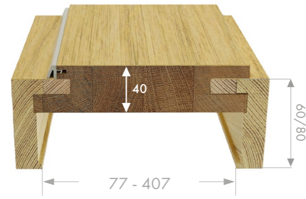
Adjustable doorframe PREMIUM
